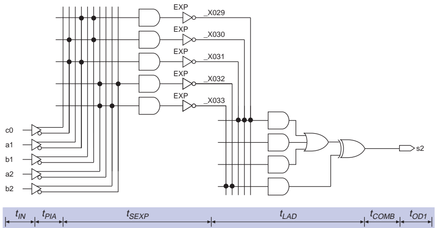
Figure 4. Adder Equations Mapped to MAX 7000 Architecture
